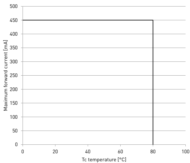
DERATING CURVE
