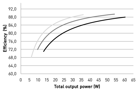
Typical efficiency
