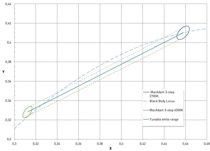
CIE 1931 Chromaticity Diagram
